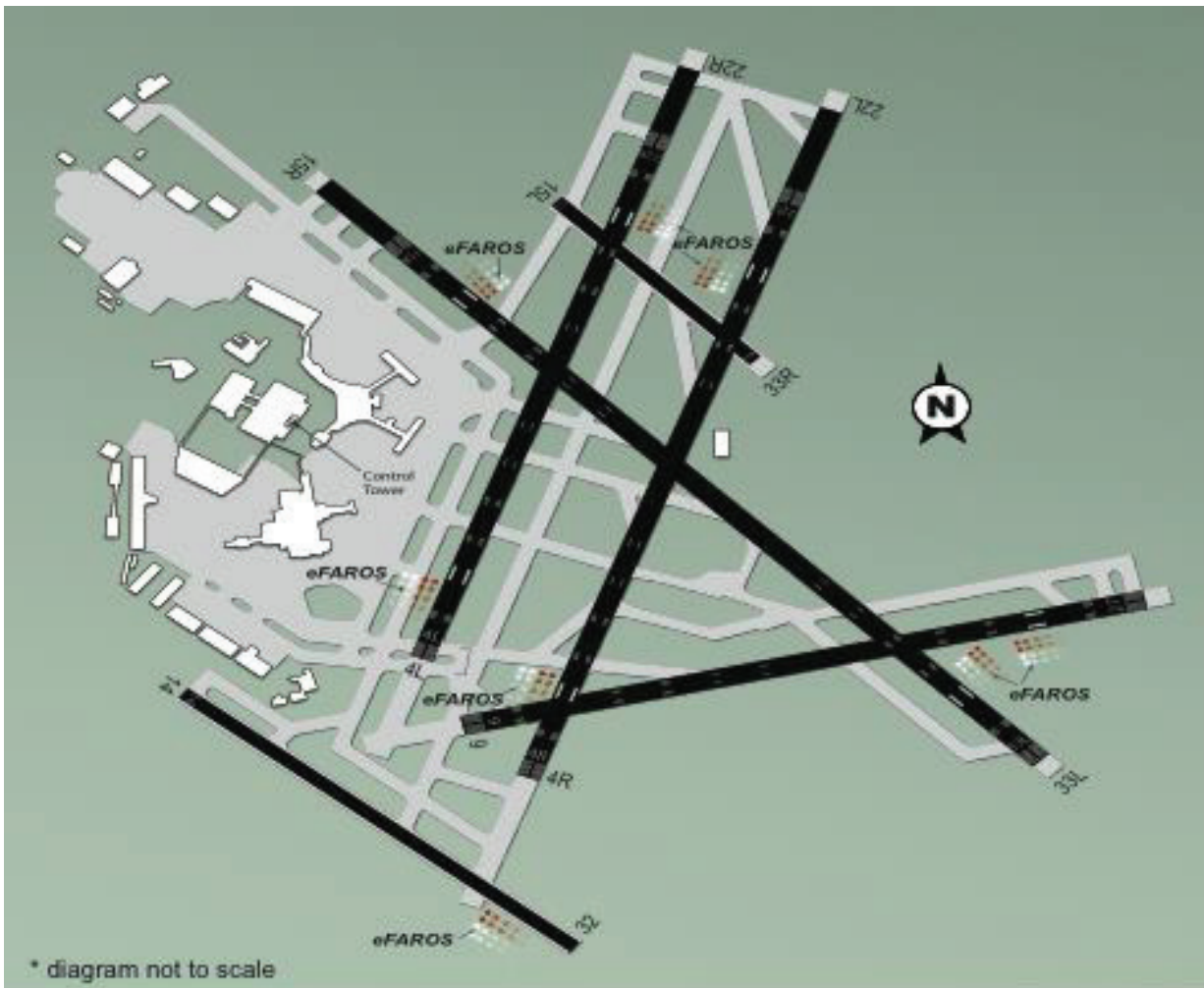
Figure 3 - eFAROS PAPI Locations
